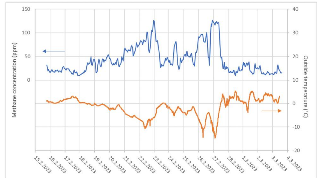
Figure 24. Wintertime long-term methane measurement inside the barn compared to outside temperature from the nearest public recording place, Turku Airport [2]. The methane concentration shown here is an average over one hour of measurement
